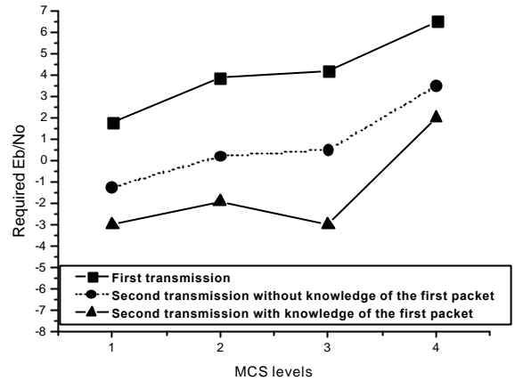
Fig. 5. Required Eb/No to satisfy a target PER of 0.01 in the Partial IR scheme
