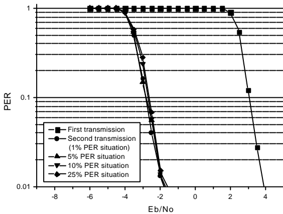
Fig. 7. PER performance of the proposed scheme in the presence of the feedback information errors
