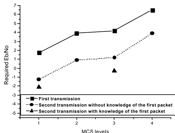
Fig. 3. Required Eb/No to satisfy a target PER of 0.01 in the Chase combining scheme
