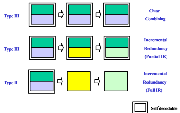
Fig. 1. Three types of HARQ schemes in HSDPA
