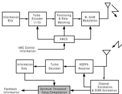
Fig. 2. Structure of the proposed scheme
